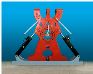
HNG 15.3 - The heavy-duty articulation system
